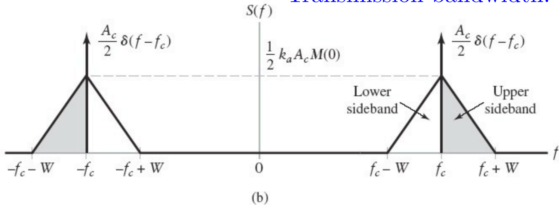
FIGURE 3.2 (a) Spectrum of message signal m(t) . (b) Spectrum of AM wave s(t) .
